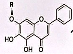
Baicalin
