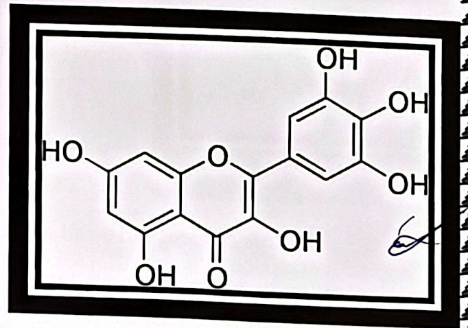
Myricetin
