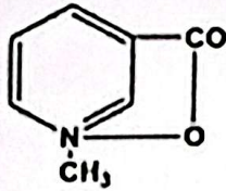
Trigonelline
